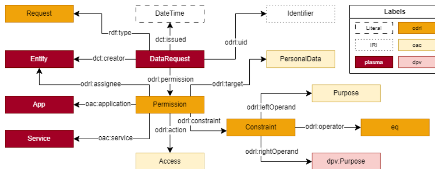
Figure 2: Ontology Design Pattern for DataRequests.
