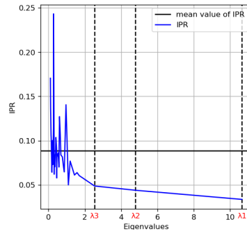
Figure 2. Inverse Participation Ratio of the empirical eigenvalues.
