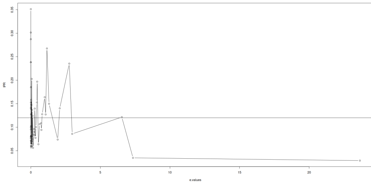
Figure 6: Inverse participation ratio (IPR) as a function of eigenvalue \lambda for the cross correlation matrix C .
