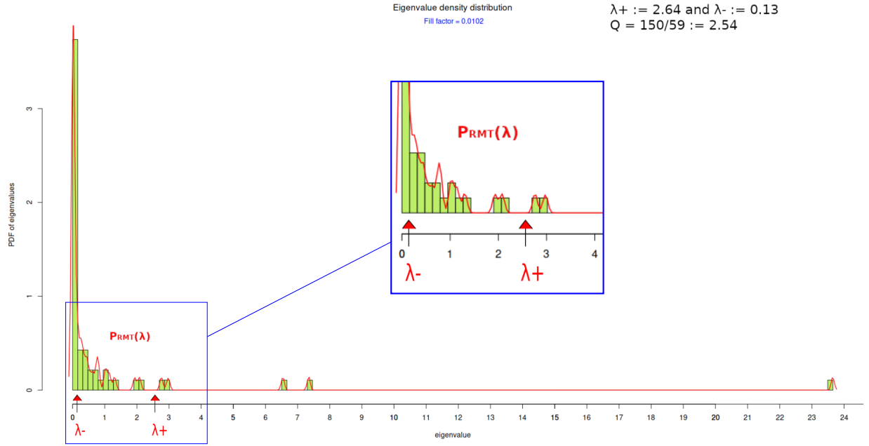
Figure 3: Eigenvalue distribution P(\lambda) for cross-correlation matrix C computed from N = 59 and L = 150
