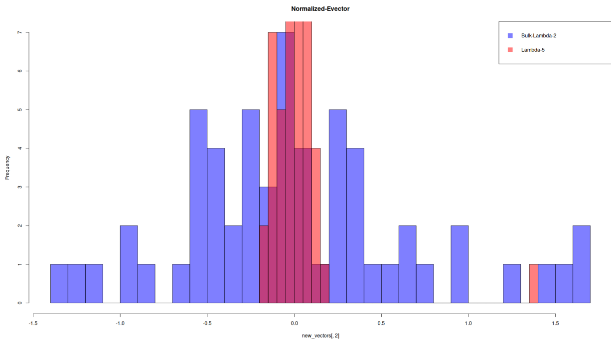
Figure 5: Distribution \rho(u) of eigenvector components for two eigenvalues, one from the bulk \lambda_- < \lambda < \lambda_+ (blue) and one from \lambda_i > \lambda_+ (red)
