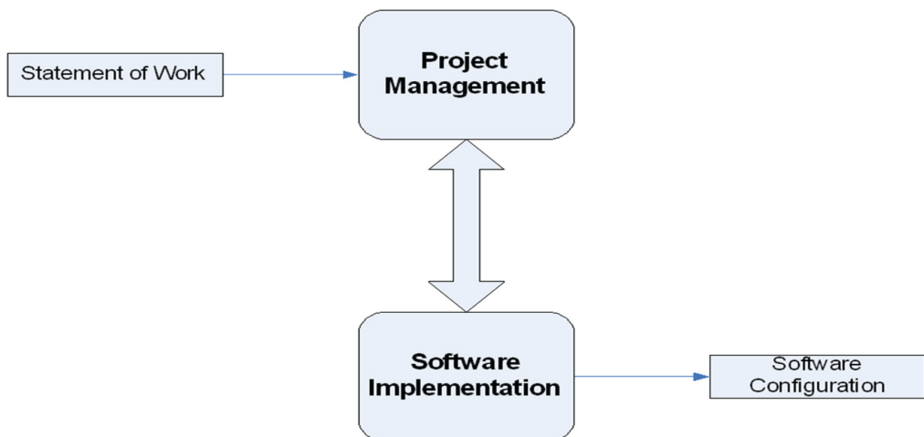
Figure 2. ISO/IEC 29110 project management and software implementation relationship
