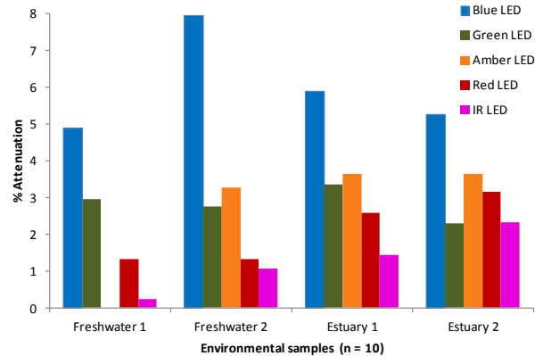
Figure 5. Field analysis of environmental samples using OCS.
